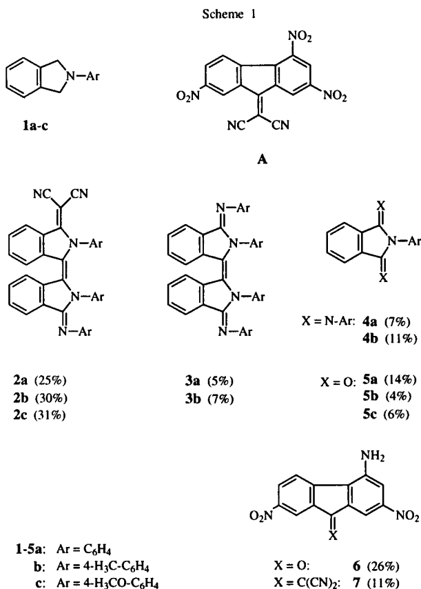
Figure 1. Molecular structure of crystalline compound 2b . The crystallographic numbering does not represent the systematic numbering.
